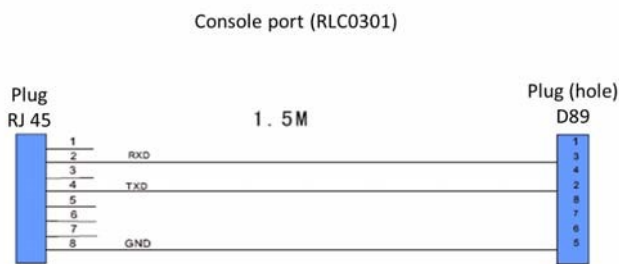
Figure 3-4 Cable connection at the console port
